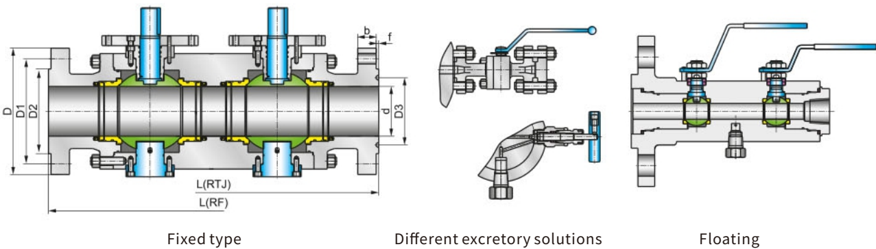
Main External Dimensions
