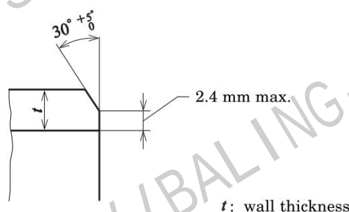
Figure 1 Shape of bevelled end
