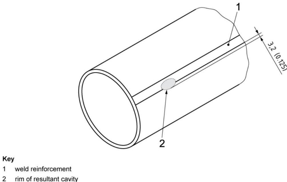
Figure C.1—Resultant Cavity of Weld Repair (PSL 2 Only)
