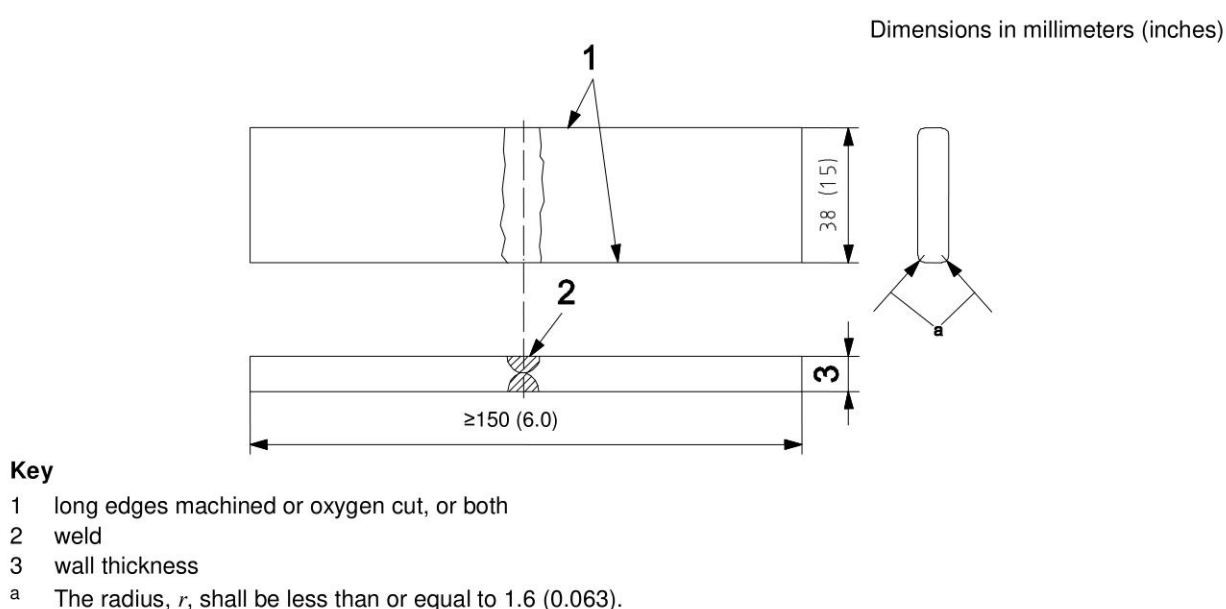
Figure 8—Guided-bend Test Pieces
