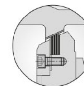
Seal Ring On The Disk
